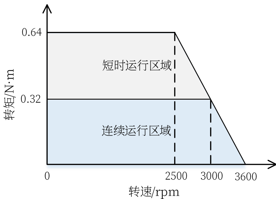
图 2-6 PMMP4010X-COE/CANopen/485-D04-X 矩频特性图 (24V, 5.98A)
