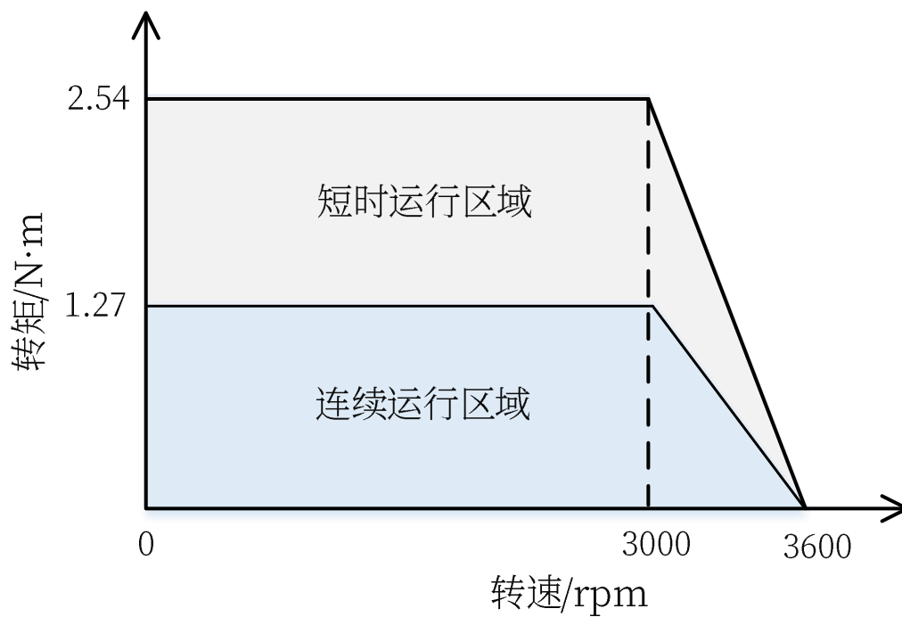
图 2-8 PMMP6040X-COE/CANopen/485-X 矩频特性图 (48V, 13.00A)
