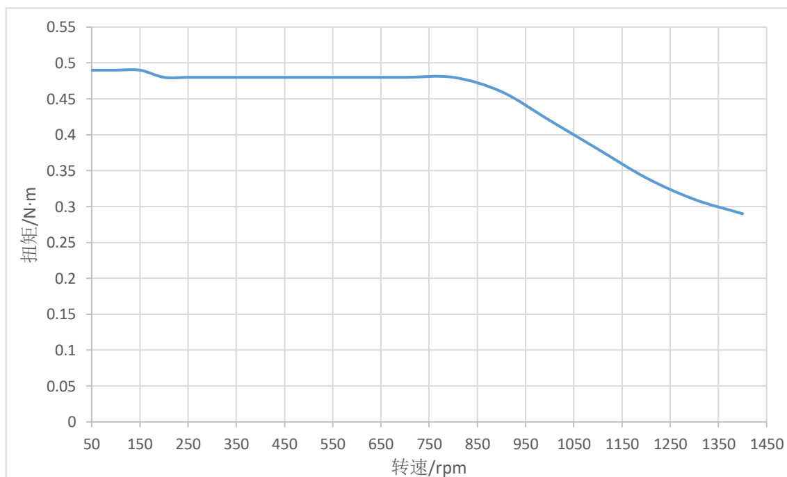
图 2-5 STM5741B-CANopen/485-ME-XX 矩频特性图 (48V, 2.8A)
