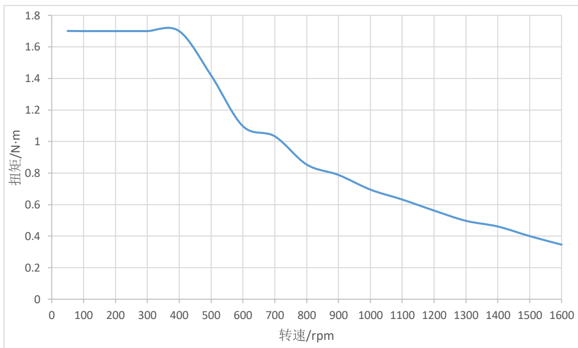
图 2-7 STM5776B-CANopen/485-ME-XX 矩频特性图 (48V, 4.2A)
