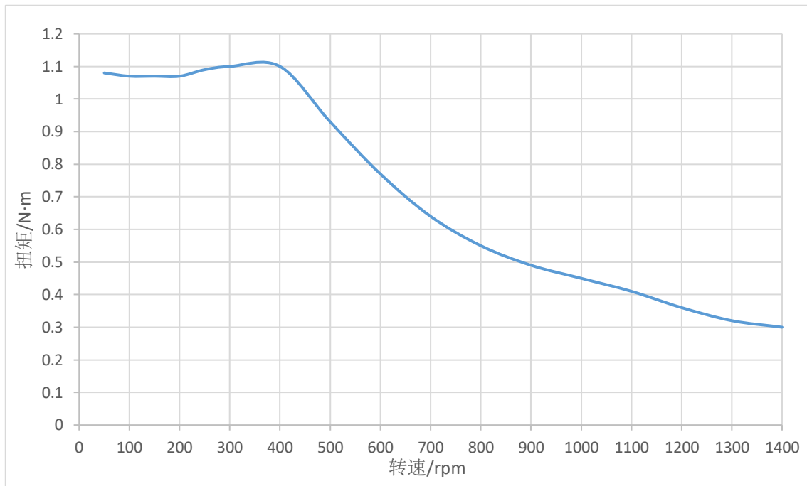
图 2-6 STM5756B-CANopen/485-ME-XX 矩频特性图 (48V, 3.0A)
