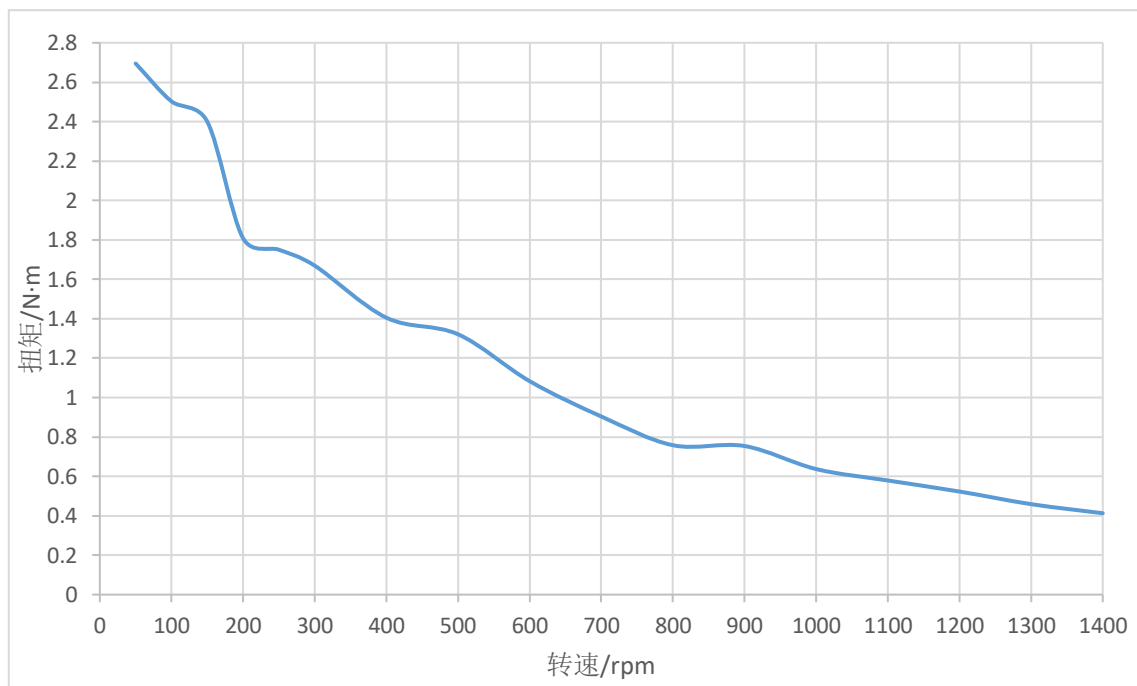
图 2-8 STM57B5B-CANopen/485-ME-XX 矩频特性图 (48V, 6.0A)
