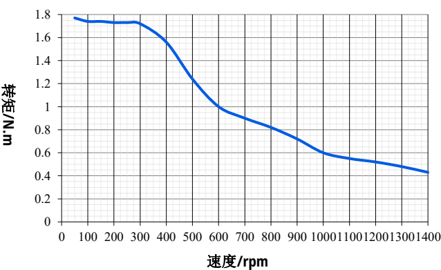
STMPW5776B-CANopen/485-XX
