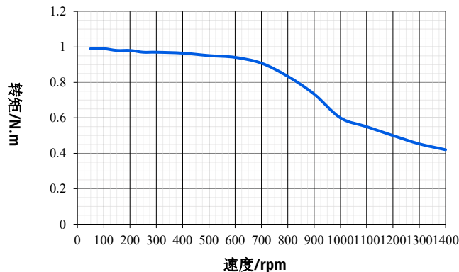
STMP5756B/D-CANopen/485
