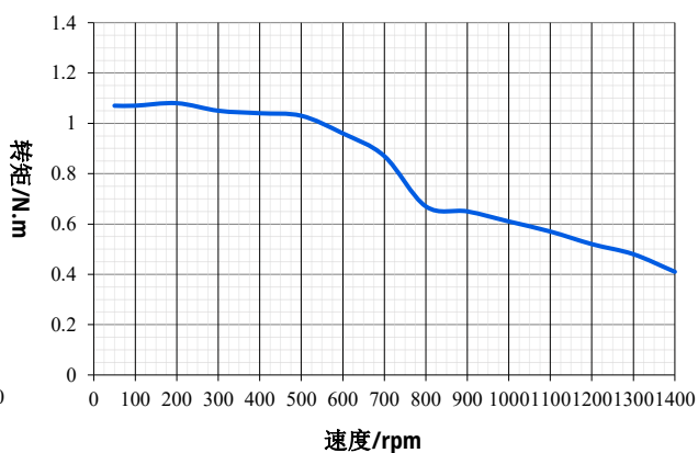
STM57B5(A)-CAN/CANopen/485-H
