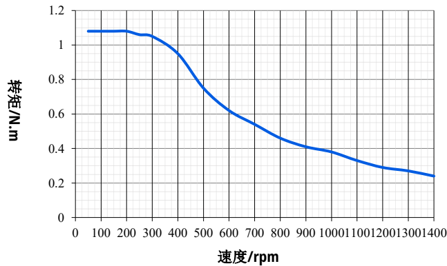
STMPW5756B-CANopen/485-XX
