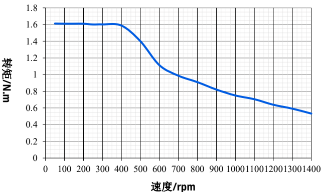
STMP5776B/D-CANopen/485
