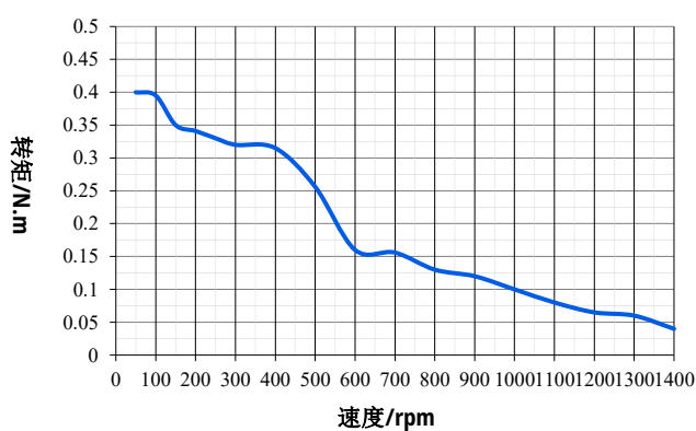
STM4240B-CANopen/485-M-XX
